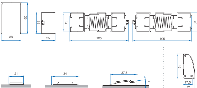
Profiles sections
